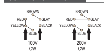
CONNECTION DIAGRAM
